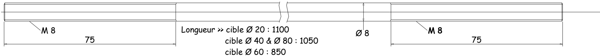
Tirants ech. 1/1
